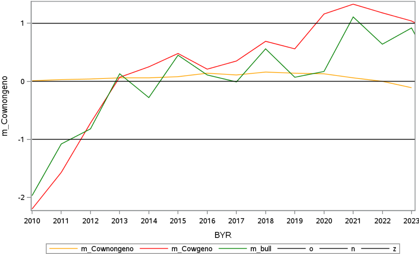
Mendelian sampling for 'ais0' 20
