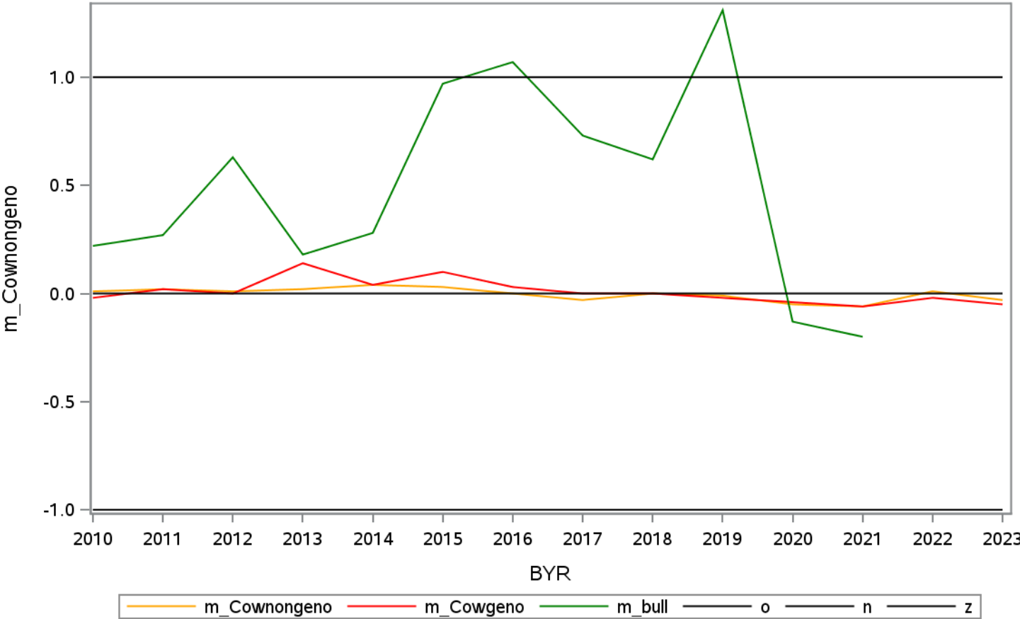
Mendelian sampling for 'ifl3' 18
