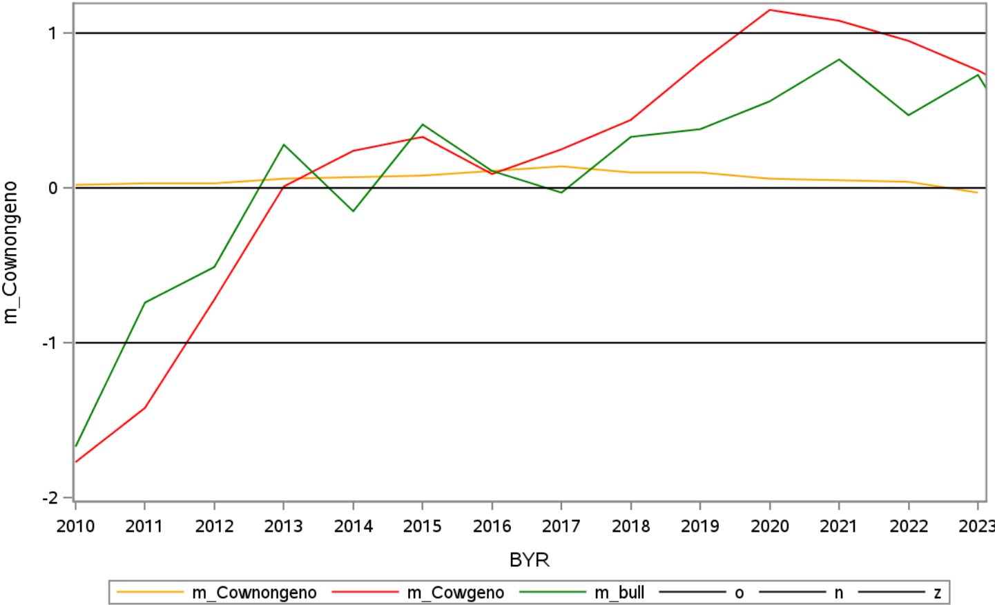
Mendelian sampling for 'nrr1' 7
