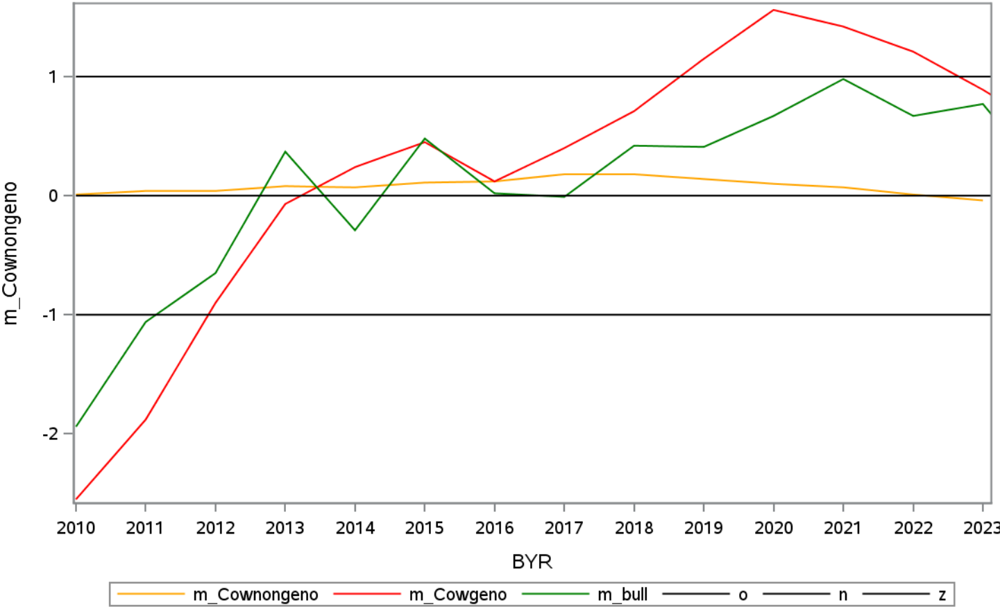
Mendelian sampling for 'fert' 34
