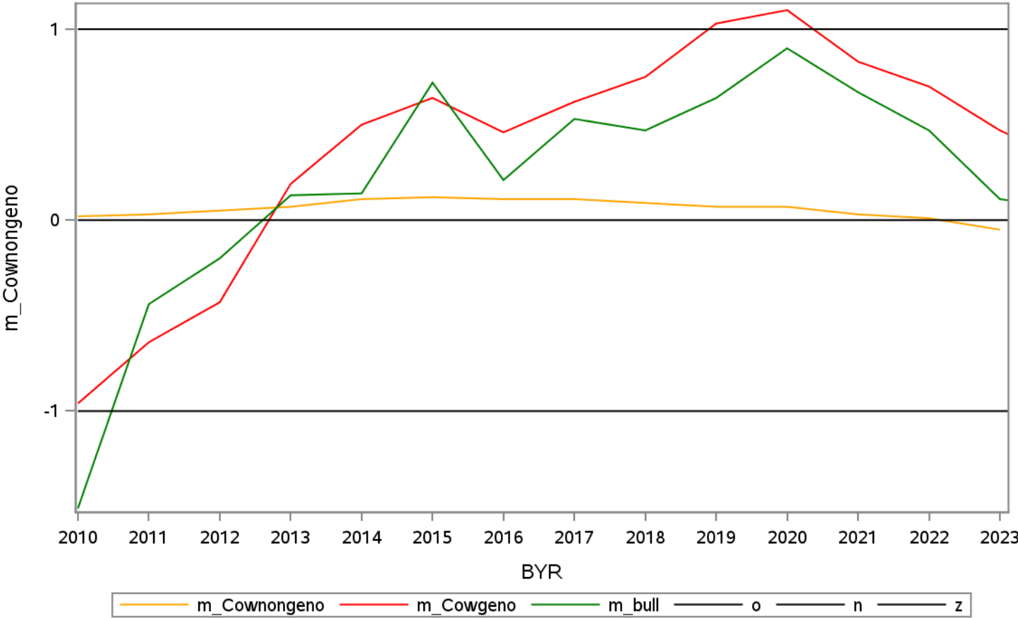
Mendelian sampling for 'cr ' 5
