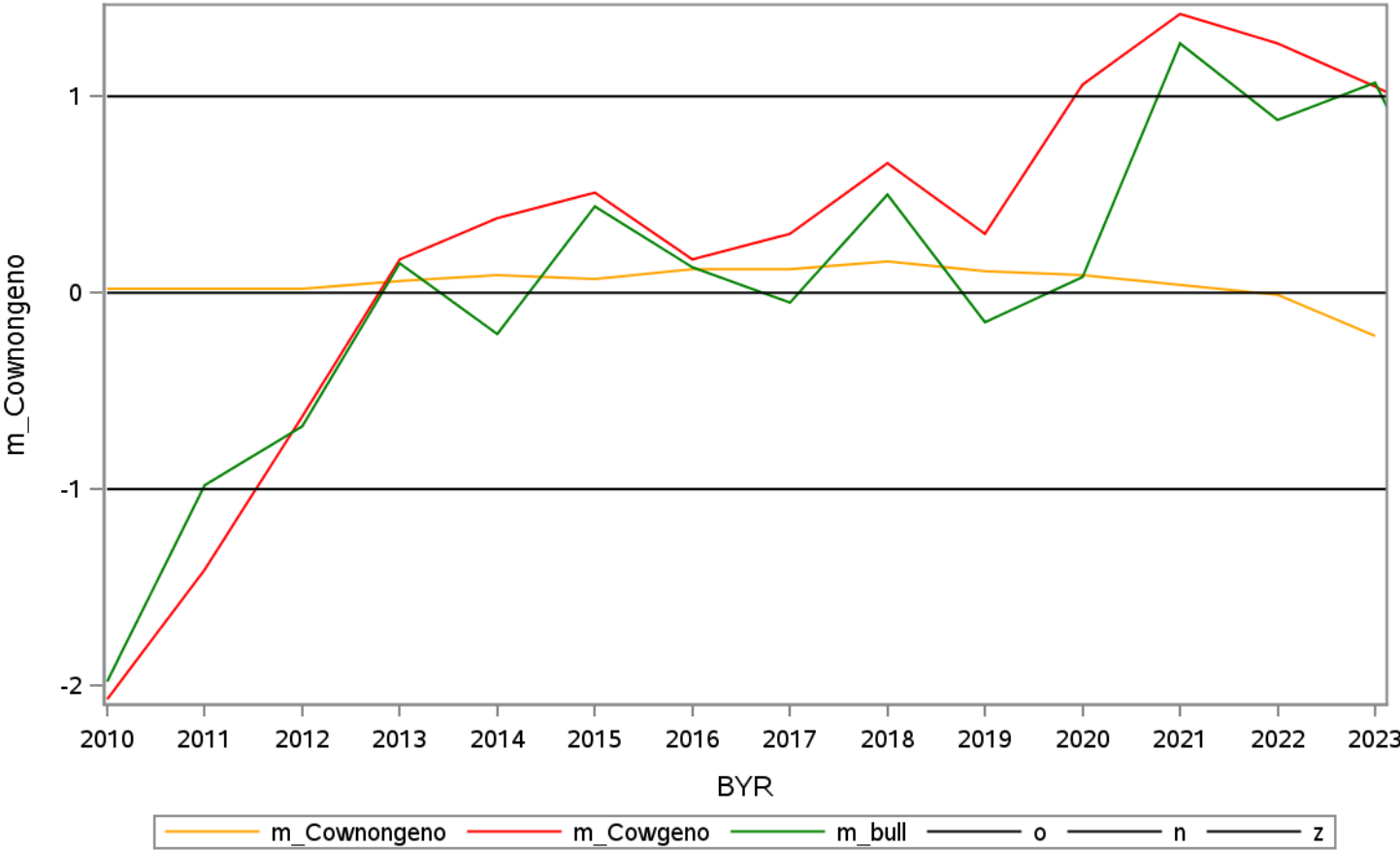
Mendelian sampling for 'nrr0' 6
