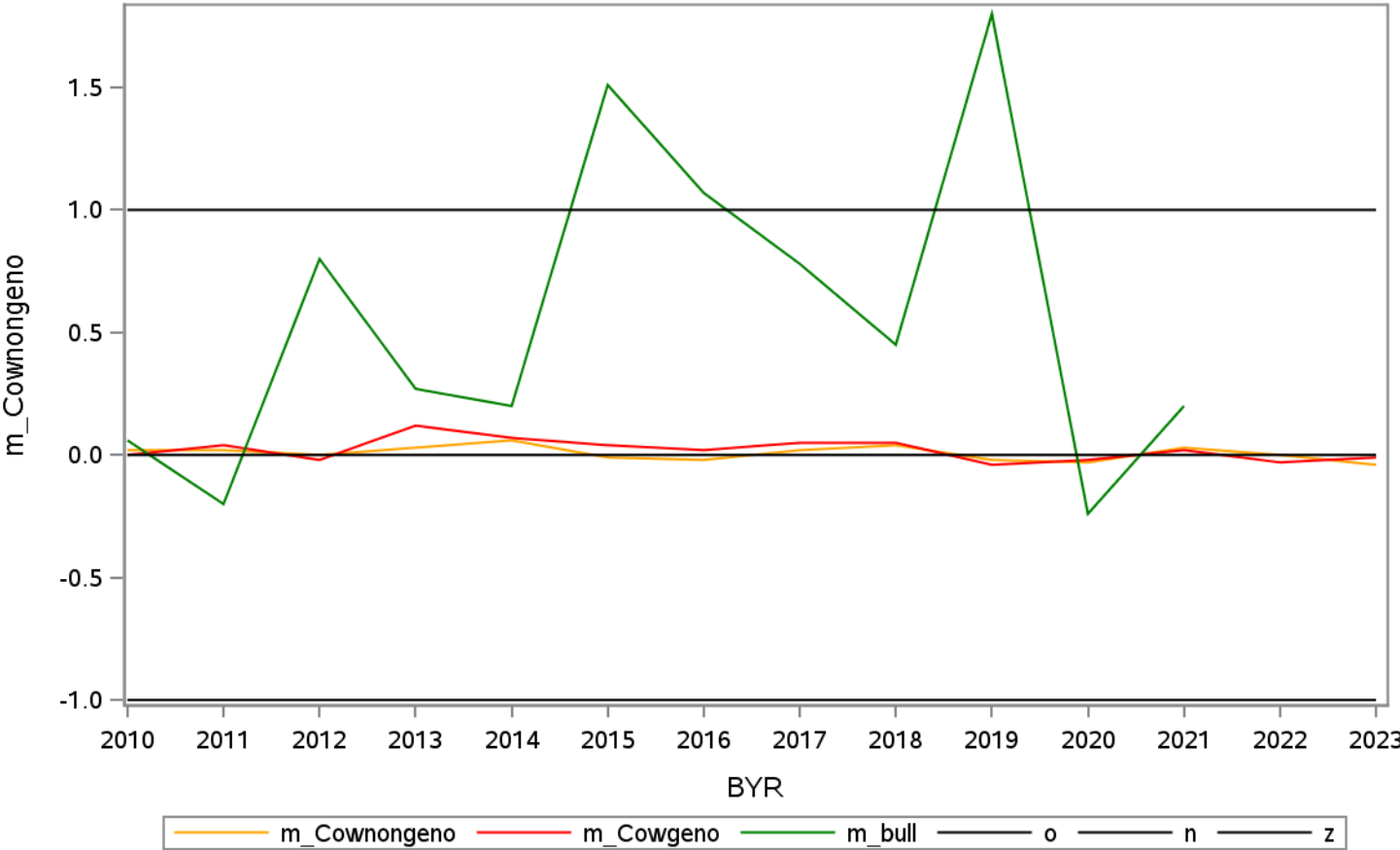
Mendelian sampling for 'ifl1' 16
