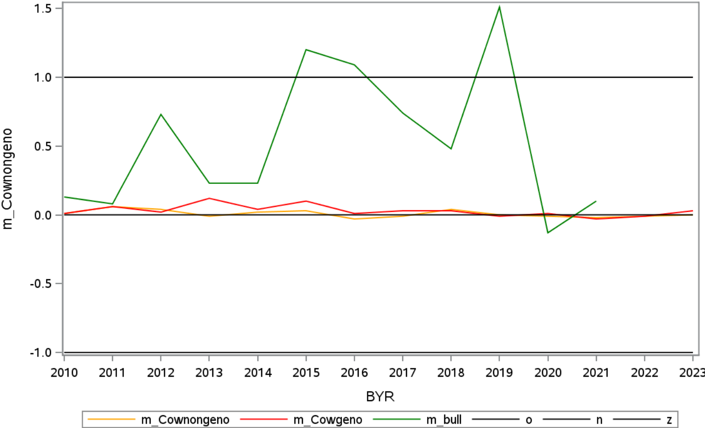
Mendelian sampling for 'ifl ' 19
