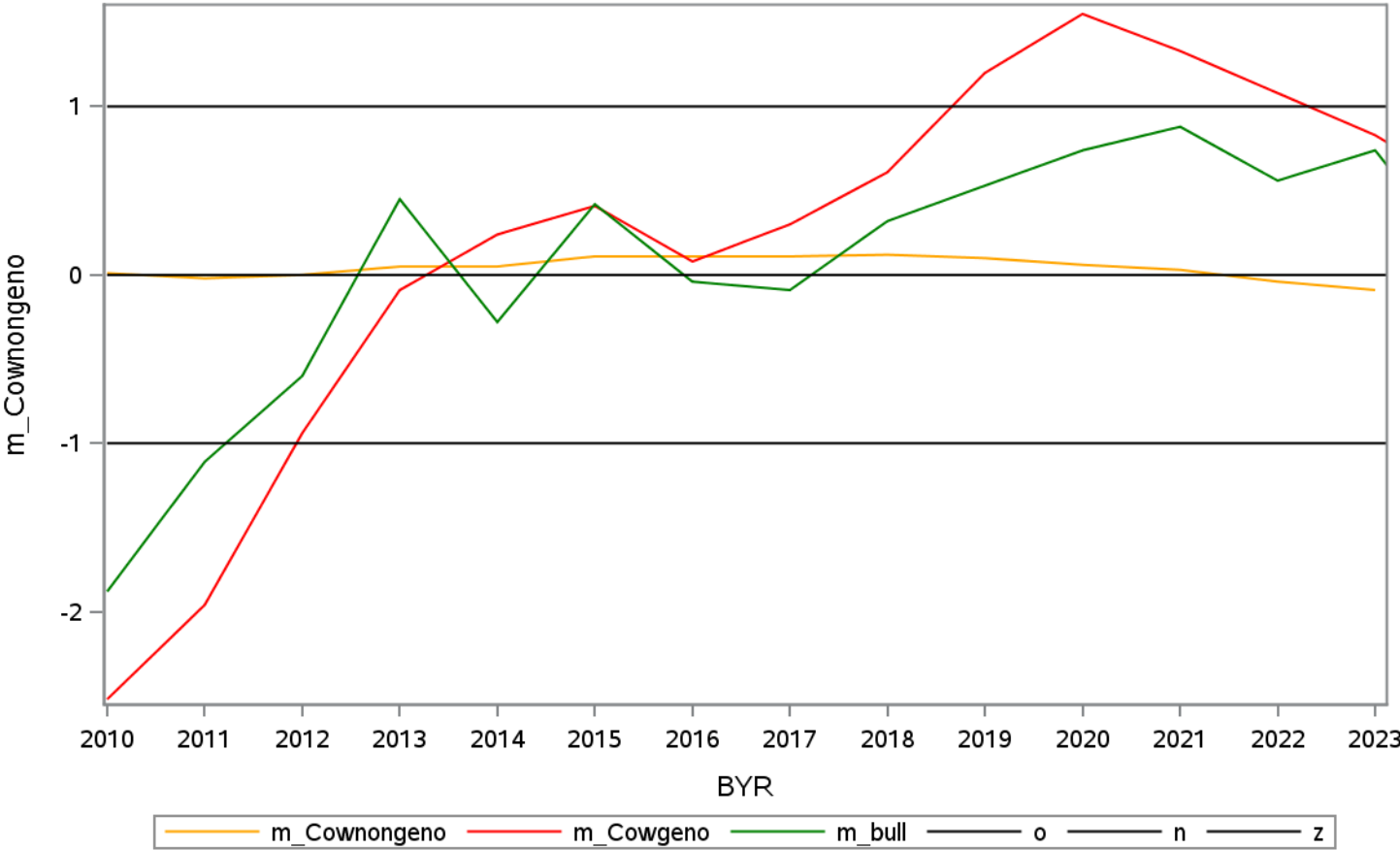
Mendelian sampling for 'ifl2' 17
