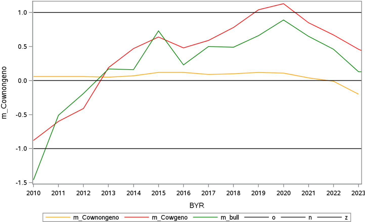
Mendelian sampling for 'cr1 ' 2
