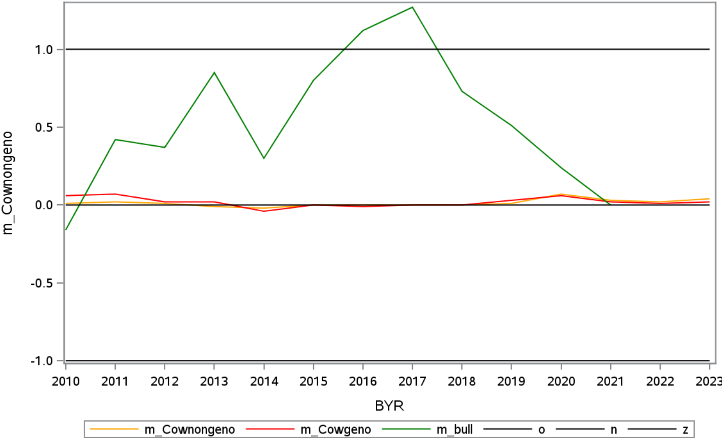
Mendelian sampling for 'cr2 ' 3
