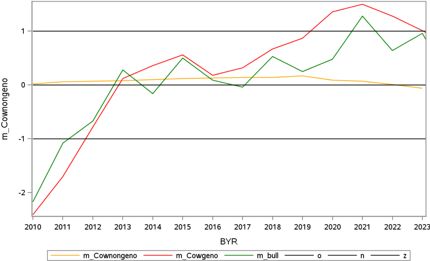
Mendelian sampling for 'cr0 ' 1
