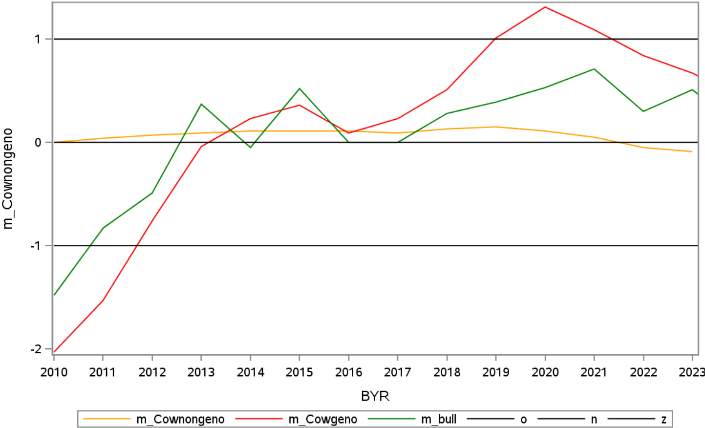
Mendelian sampling for 'ais3' 23
