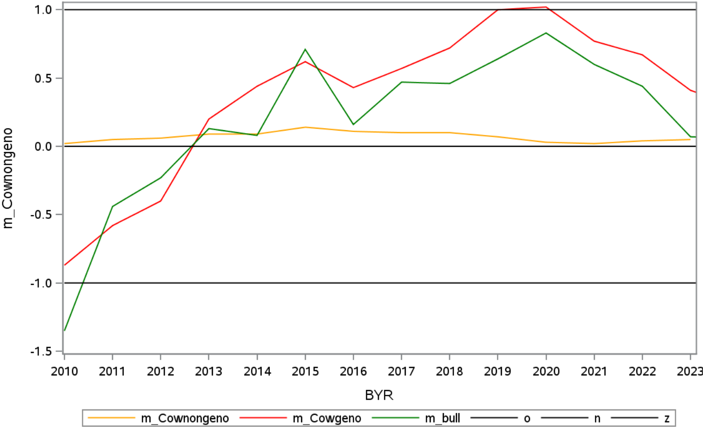
Mendelian sampling for 'cr3 ' 4
