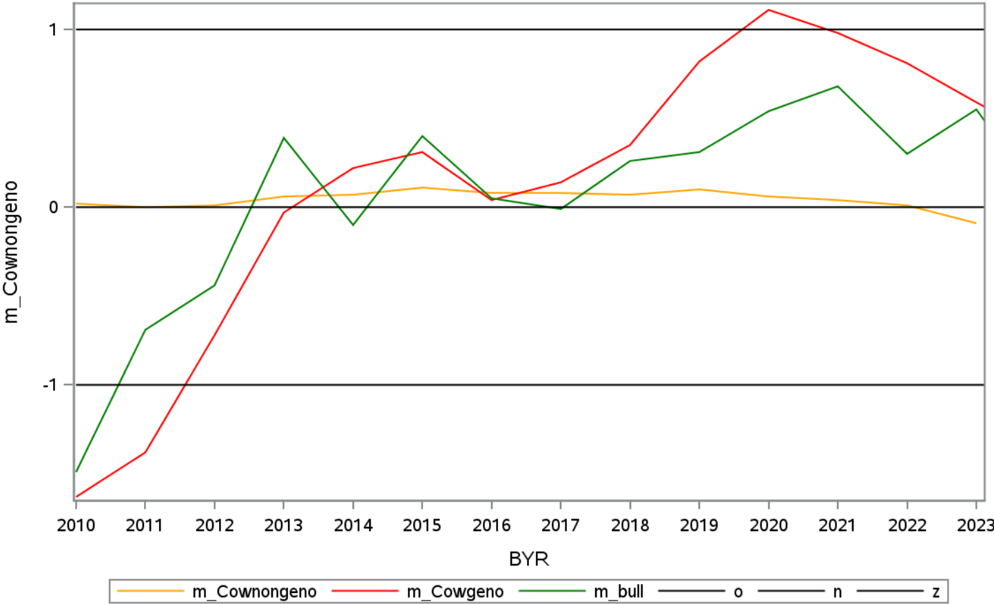
Mendelian sampling for 'nrr ' 10
