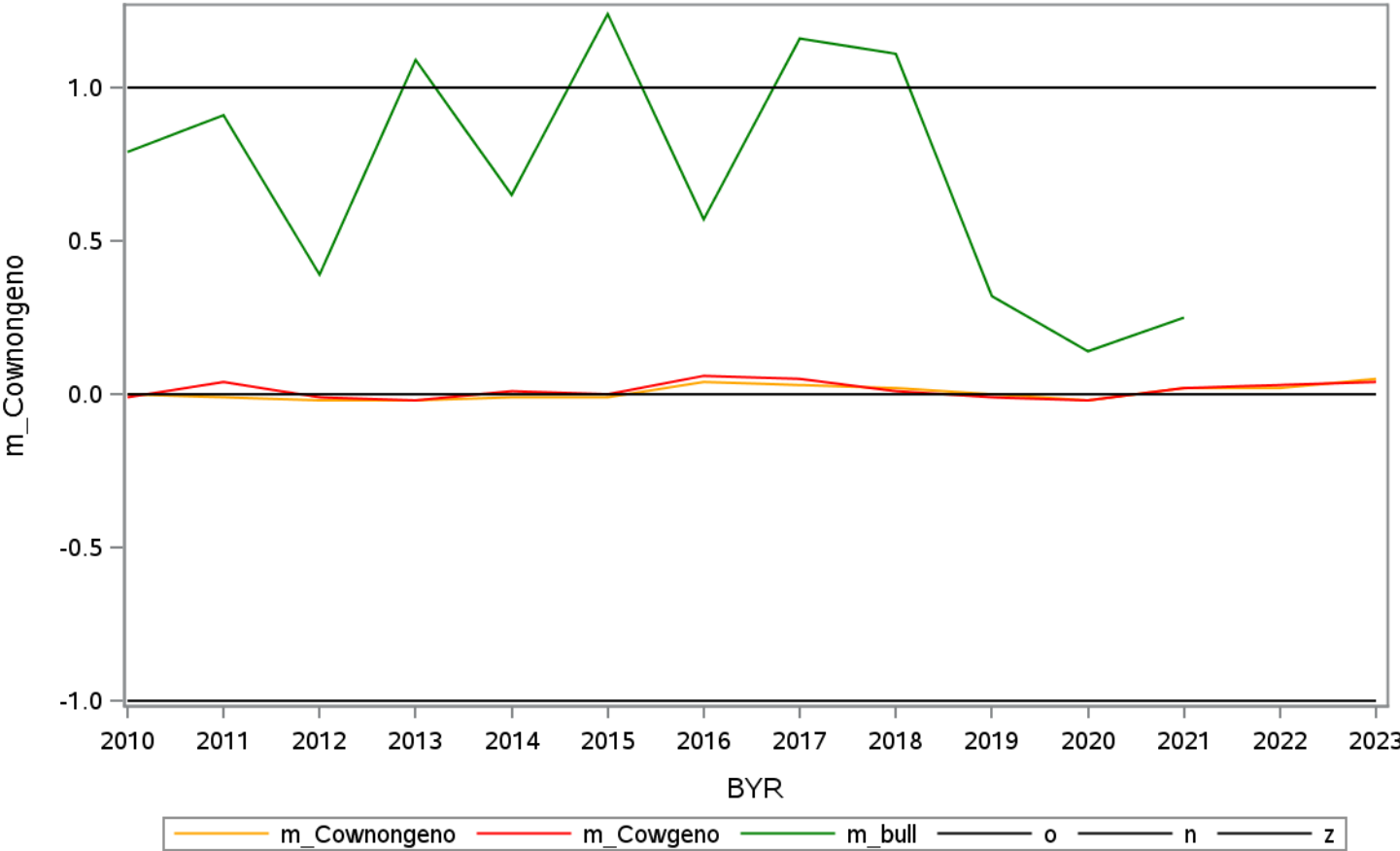
Mendelian sampling for 'nrr2' 8
