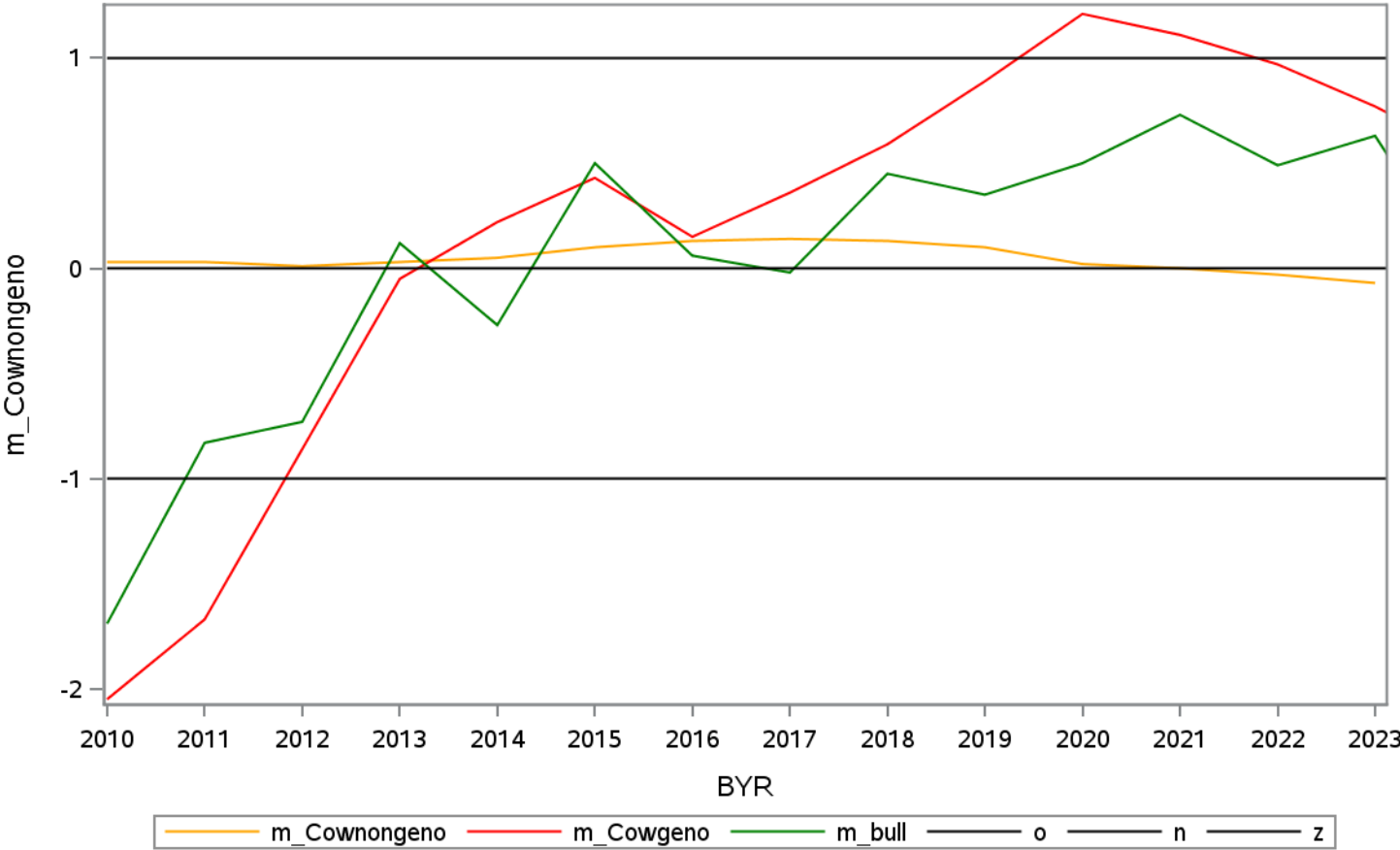
Mendelian sampling for 'ais1' 21
